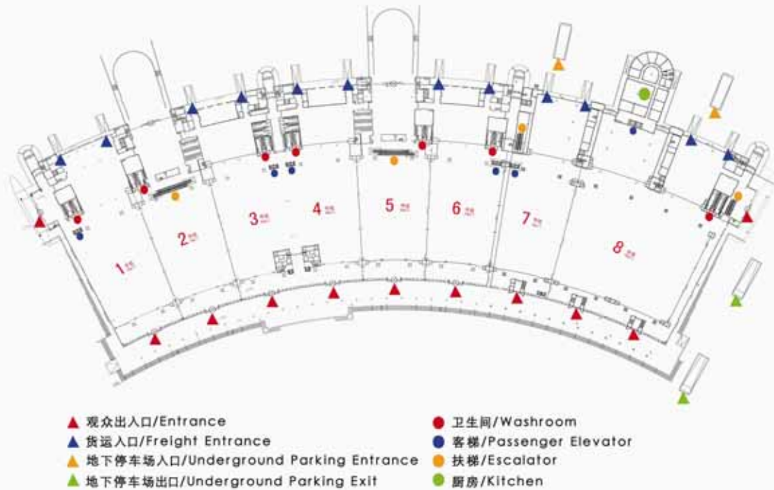
展厅平面图(一层)/layout Plan of Exhibition Hall (Level 1)
